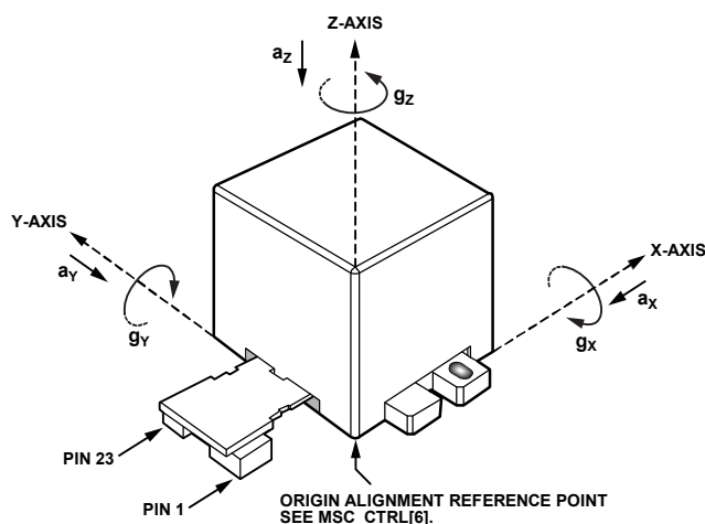
Figure 5. Pin Configuration
