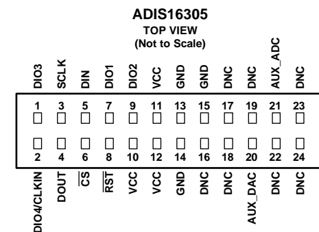
Figure 5. ADIS16305 Pin Configuration
