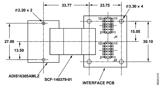
Figure 19. Physical Diagram for Mounting the ADIS16305/PCBZ
