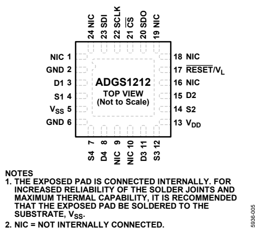
Figure 5. Pin Configuration
