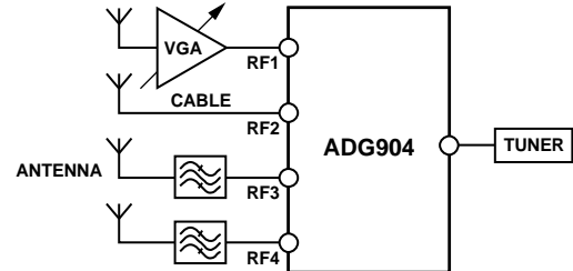
Figure 27. Tuner Modules
