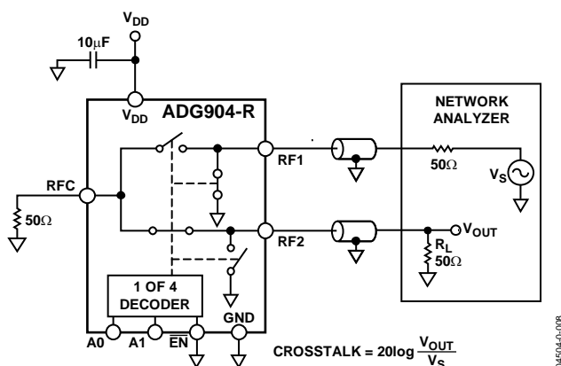
Figure 23. Crosstalk
