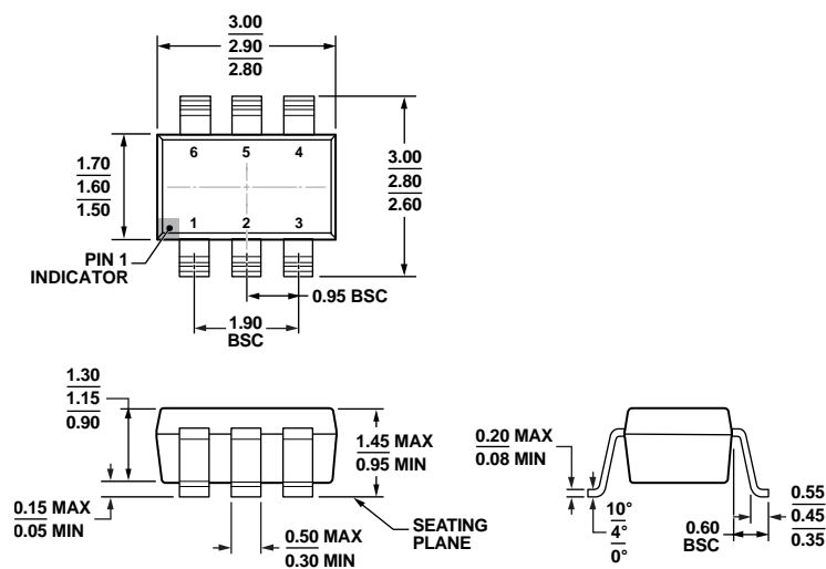
COMPLIANT TO JEDEC STANDARDS MO-178-AB Figure 19. 6-Lead Small Outline Transistor Package [SOT-23] (RJ-6) Dimensions shown in millimeters
