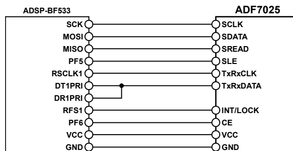
Figure 35. ADSP-BF533 to ADF7025 Connection Diagram
