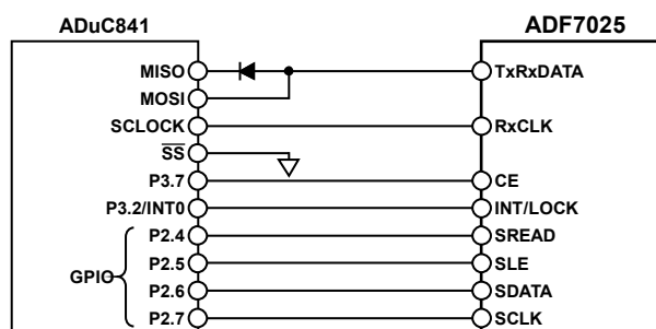
Figure 34. ADuC841 to ADF7025 Connection Diagram
