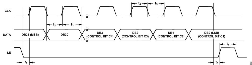
Figure 2. Write Timing Diagram
