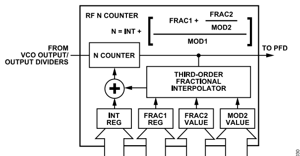
Figure 30. RF N Divider
