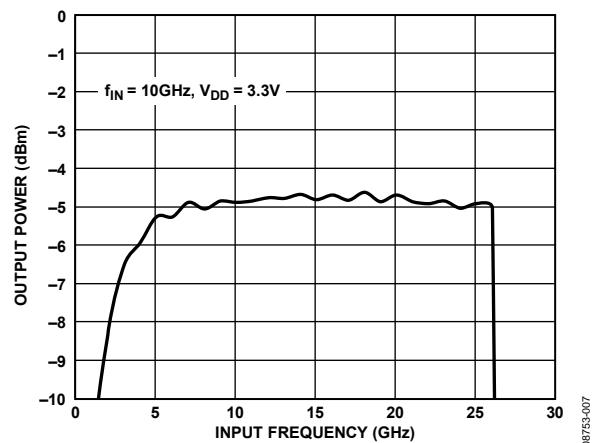
Figure 7. RF Output Power vs. RF Input Frequency, f_{IN} = 10\text{GHz} , V_{DD} = 3.3V
