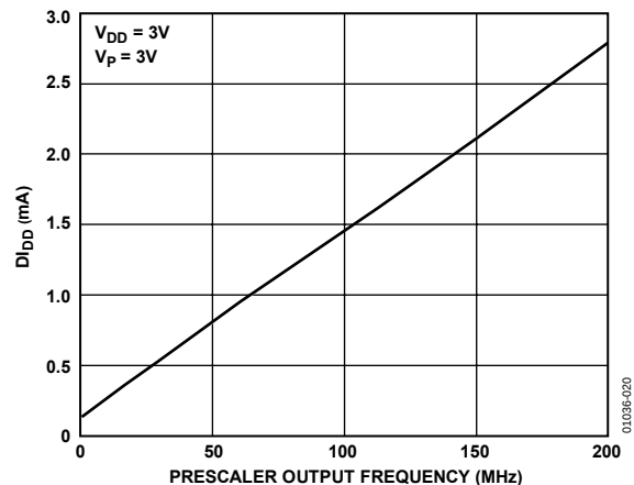
Figure 20. I_{DD} vs. Prescaler Output Frequency RF1 and RF2 (All Models)
