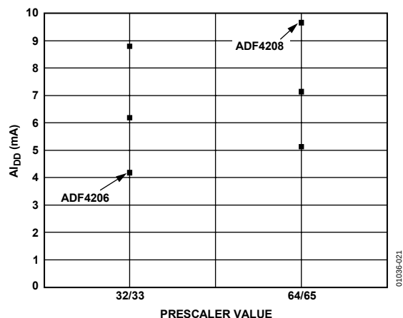
Figure 21. ADF4206/ADF4208 A_{LDD} vs. Prescaler Value (RF1)
