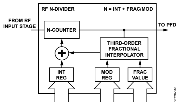
Figure 18. RF N-Divider
