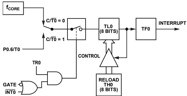
Figure 84. Timer/Counter 0, Mode 2
