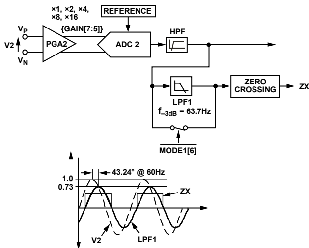
Figure 42. Zero-Crossing Detection on the Voltage Channel
