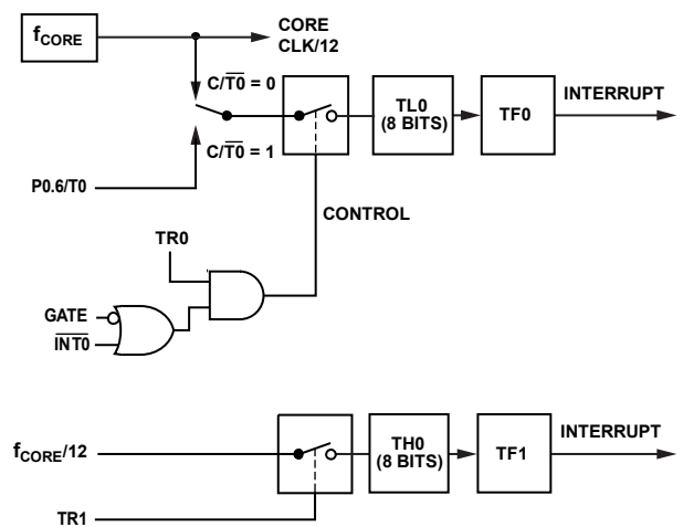
Figure 85. Timer/Counter 0, Mode 3
