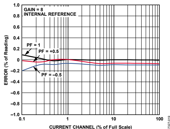
Figure 19. Reactive Energy Error as a Percentage of Reading (Gain = 8) over Power Factor with Internal Reference
