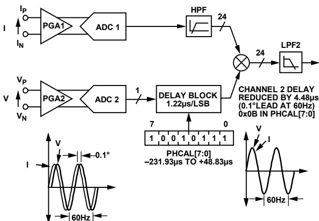
Figure 46. Phase Calibration
