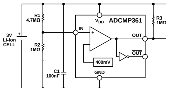
Figure 2. Typical Li-Ion Monitoring Application
