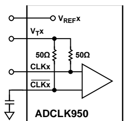
Figure 23. DC-Coupled 3.3 V CMOS Input Termination
