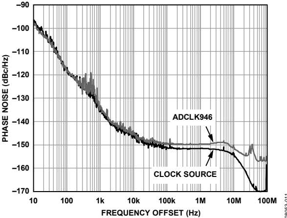
Figure 11. Absolute Phase Noise Measured @1 GHz with Agilent E5052
