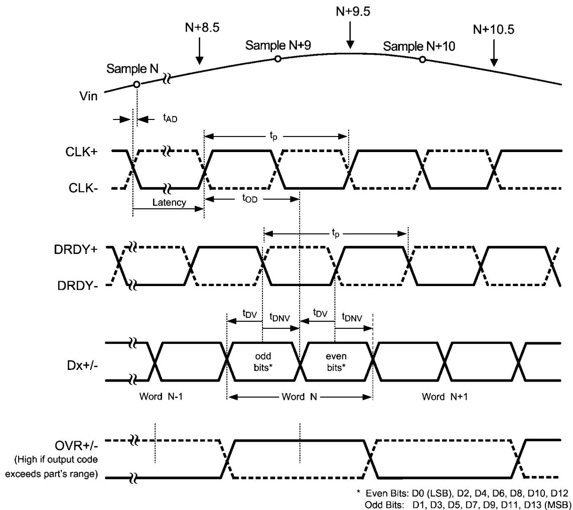
Output Timing
