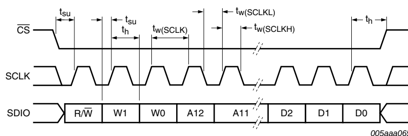
Fig 6. SPI timing
