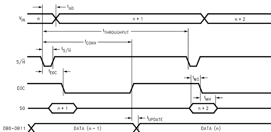
Figure 21. High Speed Interface Timing (MODE = 0, OE = 1, \overline{\text{CS}} = 0 , \overline{\text{RD}} = 0 )
