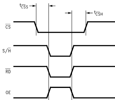
Figure 22. \overline{\text{CS}} Setup and Hold Timing for \overline{\text{S/H}} , \overline{\text{RD}} , and OE
