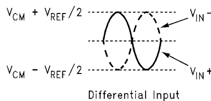
FIGURE 2. Expected Input Signal Range
