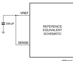
Fig 15. Internal reference via SPI, 1 V (p-p) to 2 V (p-p) full-scale
