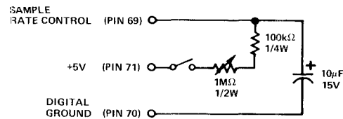
Figure 3. External Sample Rate Control Circuit
