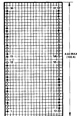
BOTTOM VIEW GRID 0.1" (2.5)
