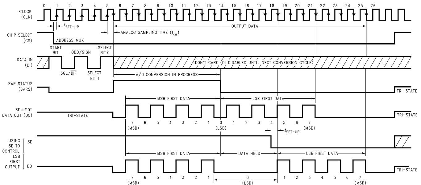
Figure 18. ADC08038 Timing
