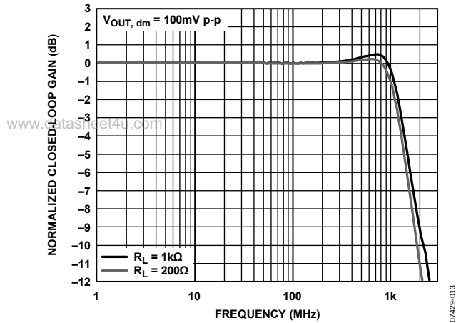
Figure 13. Small Signal Frequency Response for Various Loads
