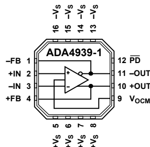
Figure 1. ADA4939-1
