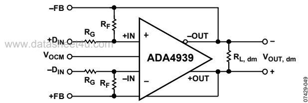
Figure 42. Circuit Definitions
