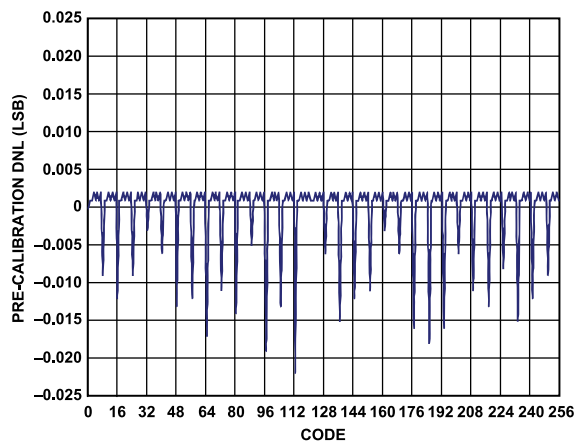
Figure 31. AD9714 Precalibration DNL at 1.8 V
