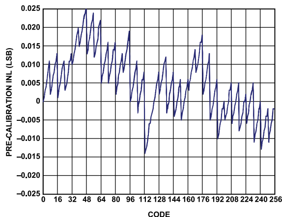
Figure 30. AD9714 Precalibration INL at 1.8 V
