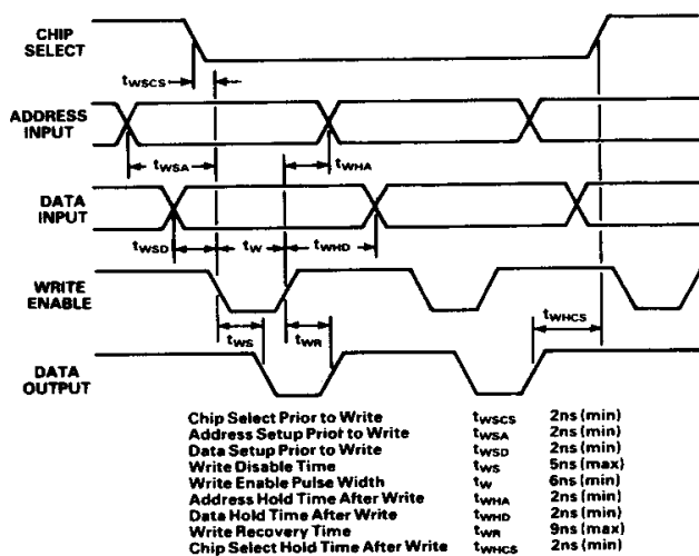
Figure 5. LUT Write Cycle Timing Diagram
