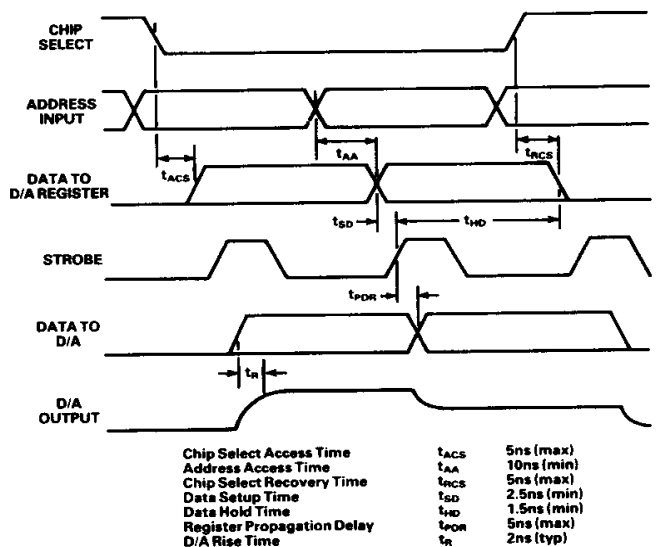
Figure 6. LUT Read Cycle Timing Diagram
