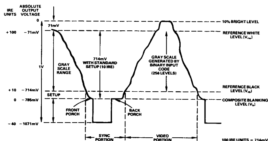
Idealized Composite Output Waveform
