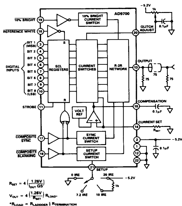
Figure 1. AD9700 D/A Connections
