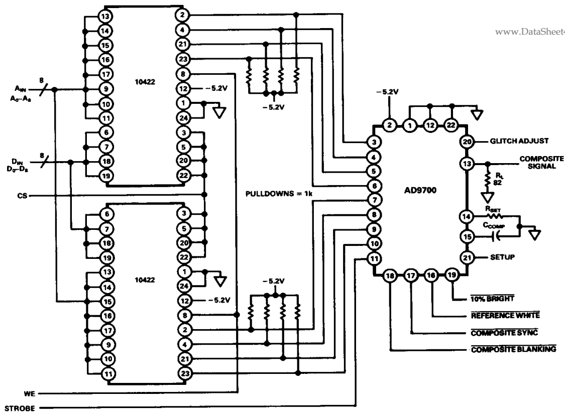
Figure 4. Using the AD9700 with Look-Up Table
