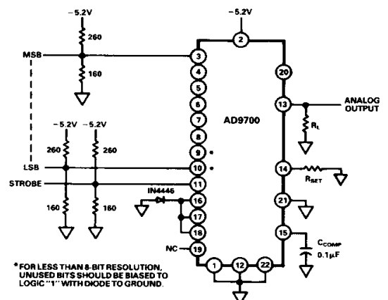
Figure 3. AD9700 as Standard D/A
