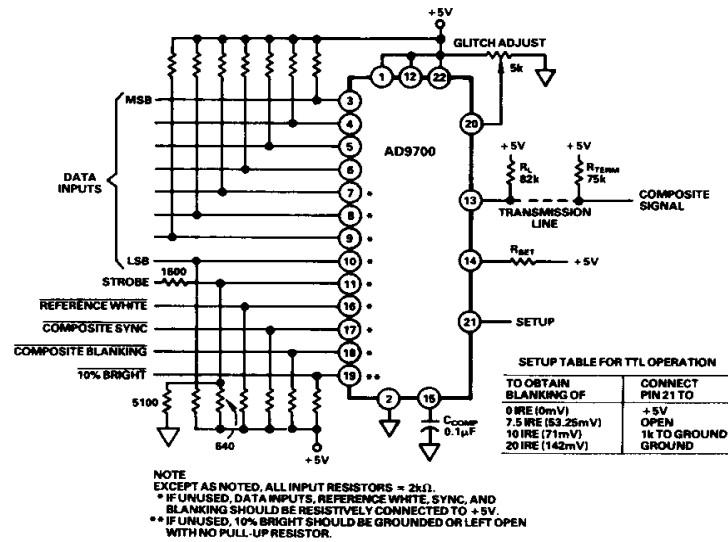
Figure 2. Using AD9700 in TTL Mode
