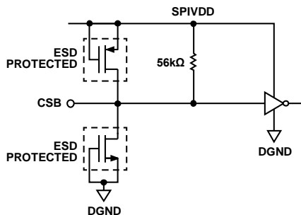
Figure 50. CSB Input
