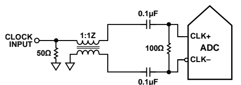
Figure 61. Transformer Coupled Differential Clock
