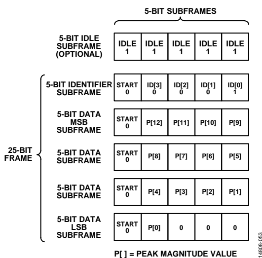
Figure 70. SPORT over JESD204B Signal Monitor Frame Data
