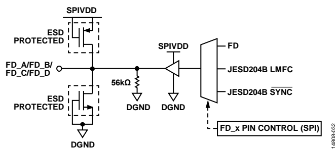
Figure 52. FD_A/FD_B/FD_C/FD_D Outputs
