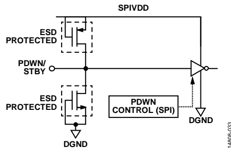
Figure 53. PDWN/STBY Input
