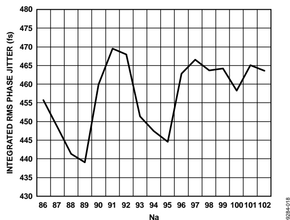
Figure 18. Typical Integrated Random Phase Jitter in fs rms for PLL1 and OUT0P LVPECL as Feedback Divider Value Na Swept ( f_{XTAL} = 25 MHz, V0 = 5 , D0 = 5 )
