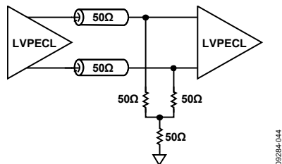
Figure 40. LVPECL DC-Coupled Y-Termination
