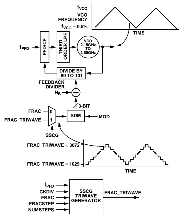
Figure 43. Spread Spectrum Clock Generator with Triangular Wave Modulation, f_{\text{PFD}} = 25 \text{ MHz}
