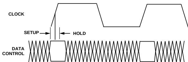
Figure 6. DATA and CONTROL Timing
