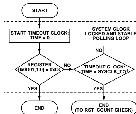
Figure 36. AD9557 System Clock Initialization Subprocess Flowchart
