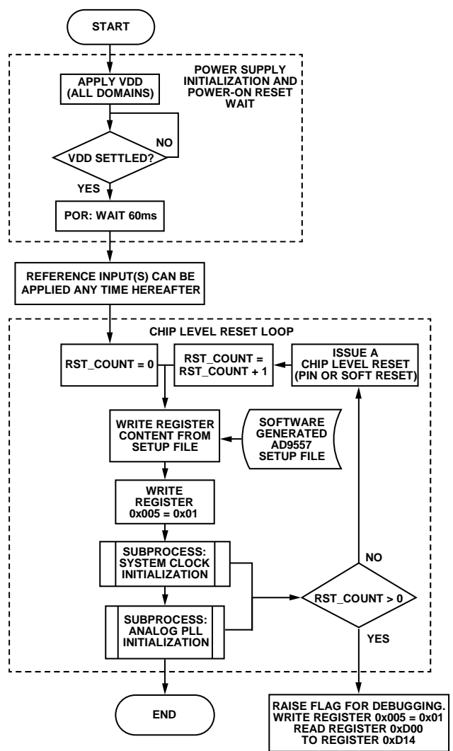
Figure 35. AD9557 Initialization Flowchart
