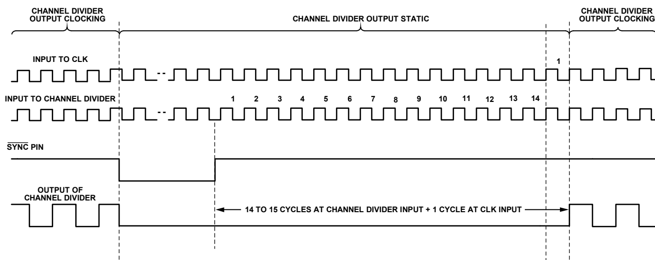
Figure 46. SYNC Timing When VCO Divider Is Not Used—CLK Input Only
