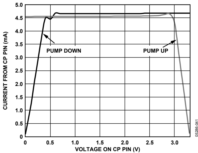
Figure 14. Charge Pump Output Characteristics @ VCP 5 = 3.3 V
