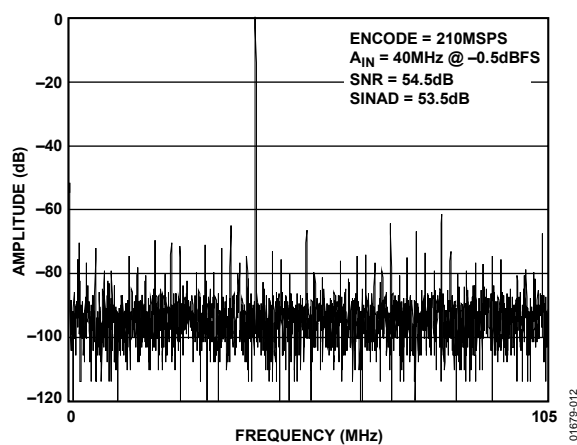
Figure 12. Single Tone at 40 MHz; 210 MSPS
