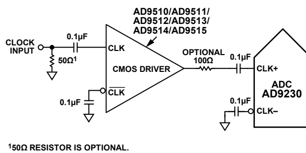
Figure 59. Single-Ended 3.3 V CMOS Sample Clock
