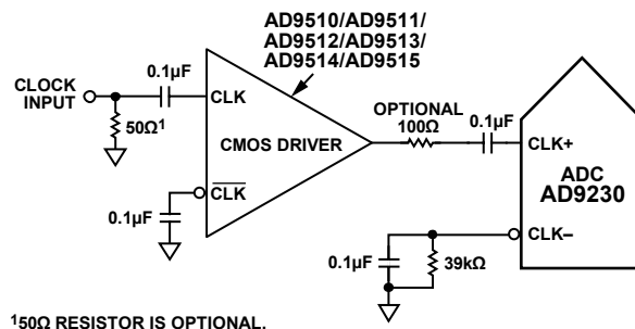
Figure 58. Single-Ended 1.8 V CMOS Sample Clock
