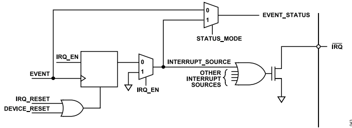
Figure 74. Simplified Schematic of \overline{\text{IRQ}} Circuitry
