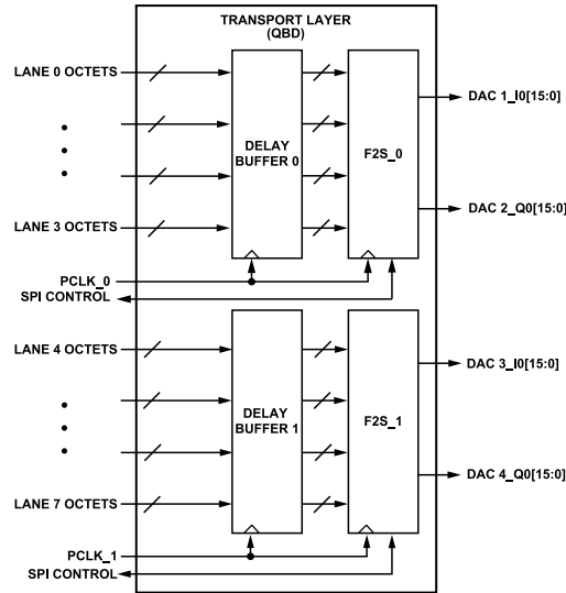
Figure 57. Transport Layer Block Diagram
