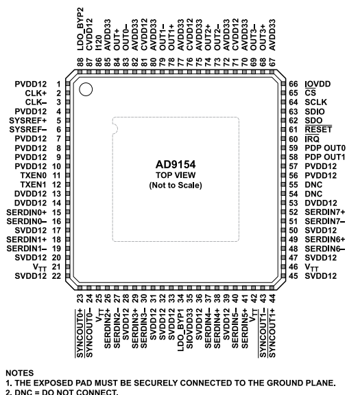
Figure 3. Pin Configuration
