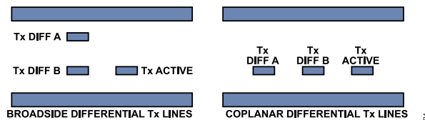
Figure 86. Broadside vs. Coplanar Differential Stripline Routing Techniques
