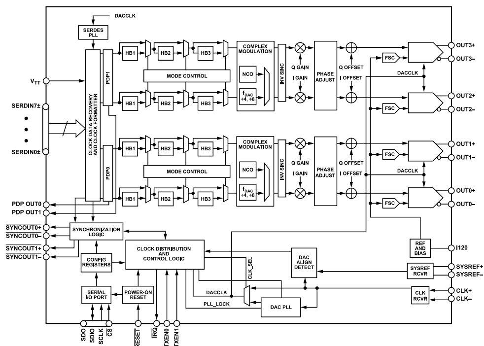
Figure 2. Detailed Functional Block Diagram
