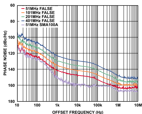
Figure 33. Single Tone Phase Noise vs. Offset Frequency at Four Different f_{OUT} Rates, f_{DAC} = 2.0 GHz, PLL Off
