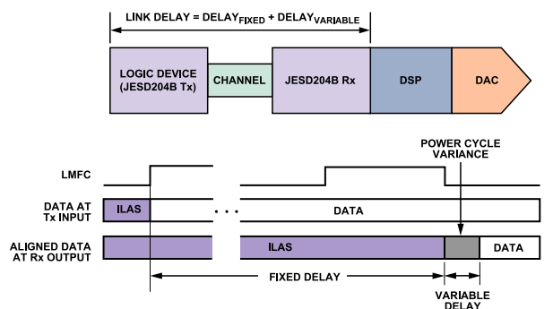
Figure 53. JESD204B Link Delay = Fixed Delay + Variable Delay
