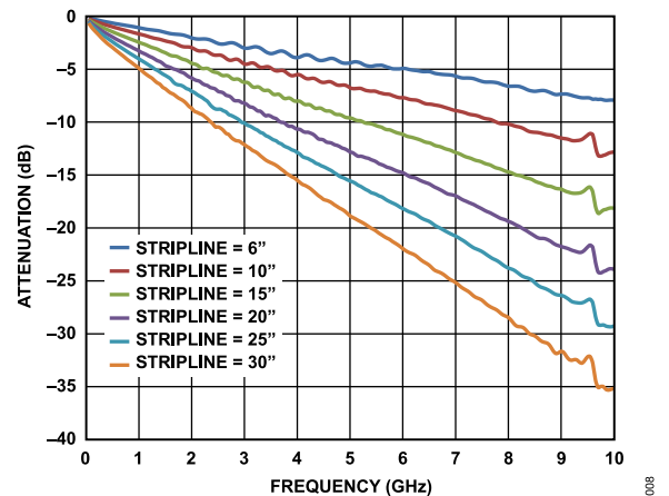
Figure 45. Insertion Loss of 50 \Omega Striplines on FR-4
