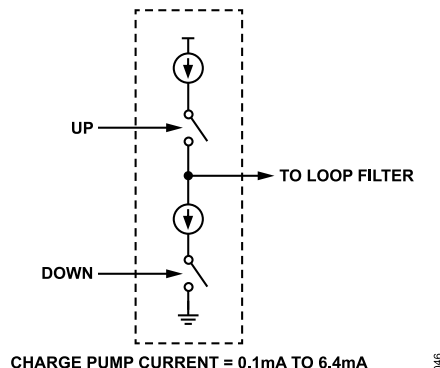
Figure 77. Charge Pump
