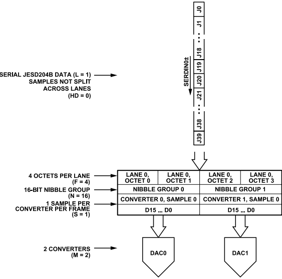
Figure 65. JESD204B Mode 7 Data Deframing
