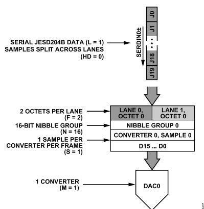
Figure 67. JESD204B Mode 10 Data Deframing
