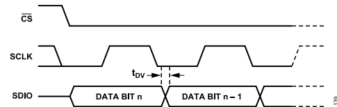
Figure 39. Timing Diagram for Serial Port Register Read
