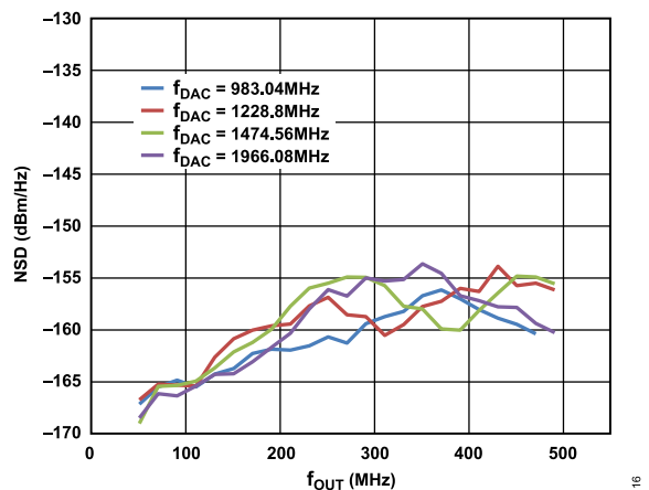
Figure 16. Single Tone (0 dBFS) NSD vs. f_{OUT} over f_{DAC} , 20 MHz Offset from Carrier
