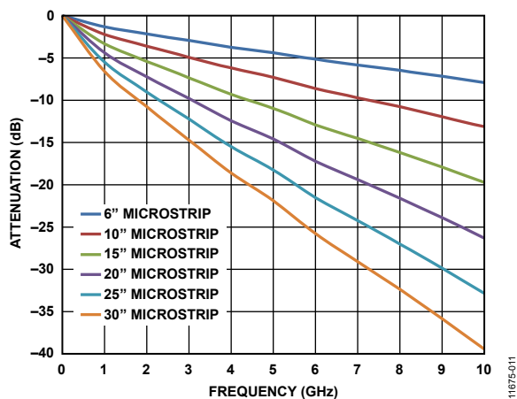
Figure 41. Insertion Loss of 50 \Omega Microstrips on FR4
