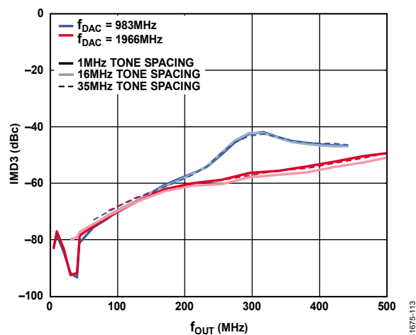
Figure 13. Two-Tone Third IMD (IMD3) vs. f_{OUT} over Tone Spacing at 0 dB Back Off, f_{DAC} = 983 MHz and 1966 MHz
