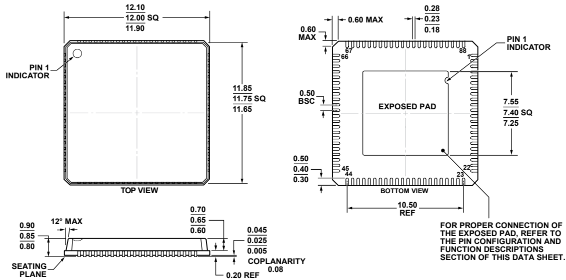
Figure 88. 88-Lead Lead Frame Chip Scale Package [LFCSP_VQ] 12 mm x 12 mm Body, Very Thin Quad (CP-88-6)
