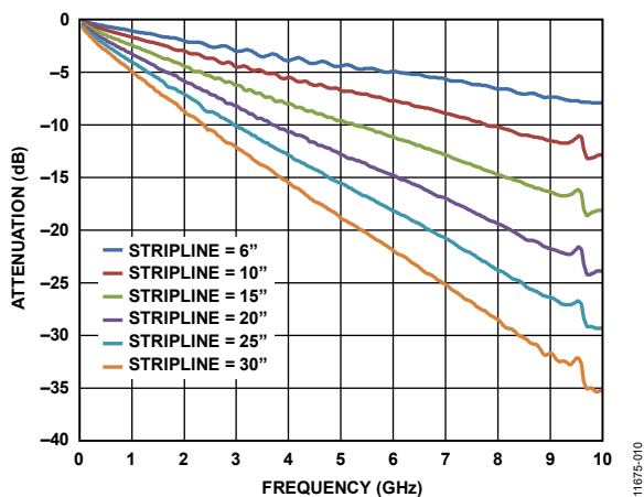
Figure 40. Insertion Loss of 50 \Omega Striplines on FR4
