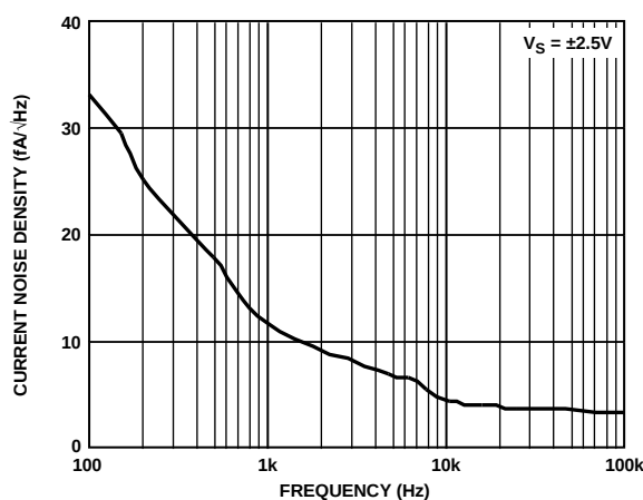
Figure 21. Current Noise Density vs. Frequency
