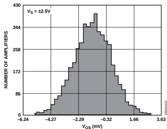
Figure 12. V_{OS} Distribution
