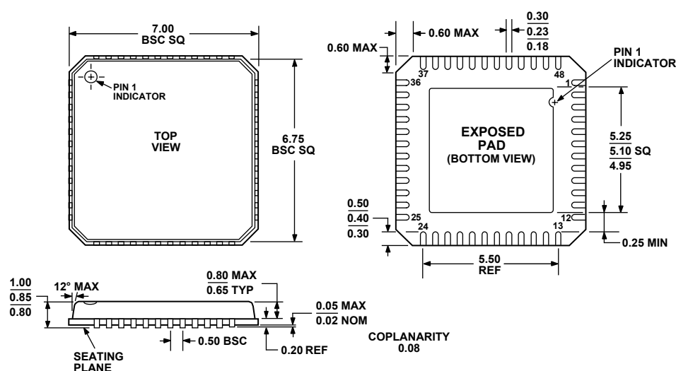
Figure 15. 48-Lead Lead Frame Chip Scale Package [LFCSP_VQ] 7 mm x 7 mm Body, Very Thin Quad
