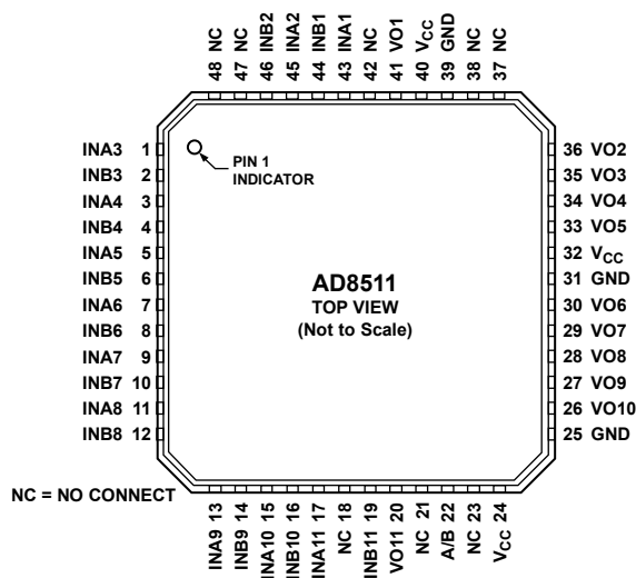
Figure 6. AD8511 (48-Lead LFCSP)
