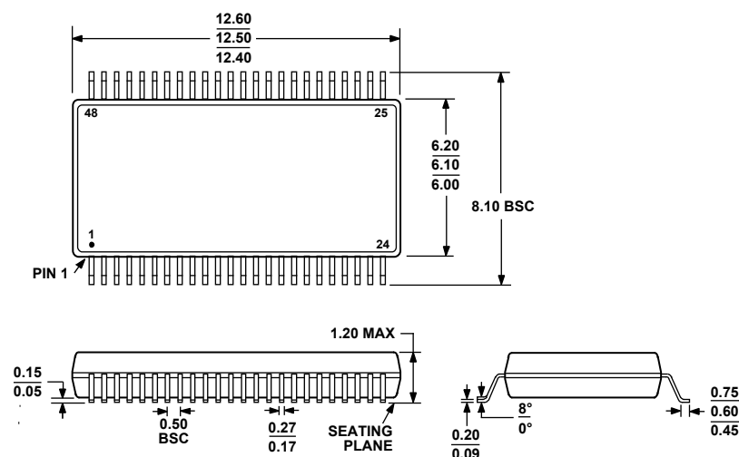
Figure 14. 48-Lead Thin Shrink Small Outline Package [TSSOP] (RV-48)
