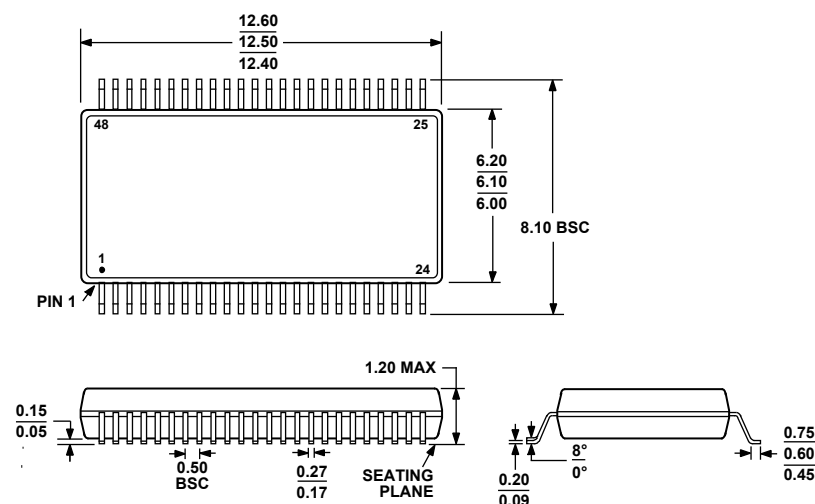
Figure 14. 48-Lead Thin Shrink Small Outline Package [TSSOP]
