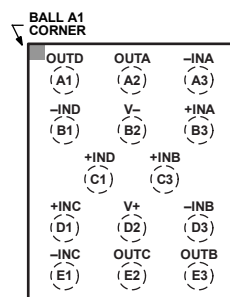
AD8508 TOP VIEW (BALL SIDE DOWN) Not to Scale
