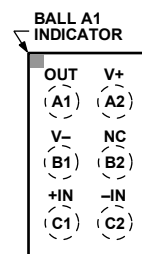
AD8505 TOP VIEW (BALL SIDE DOWN) Not to Scale NC = NO CONNECT
