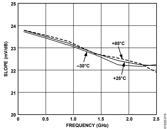
Figure 16. Slope vs. Frequency; -30^{\circ}\text{C} , +25^{\circ}\text{C} , and +85^{\circ}\text{C}
