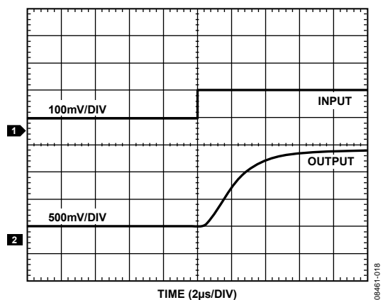
Figure 14. Rise Time
