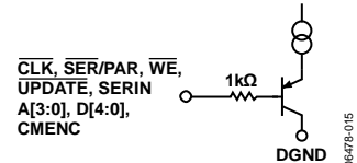
Figure 16. Logic Input (see also ESD Protection Map, Figure 19)
