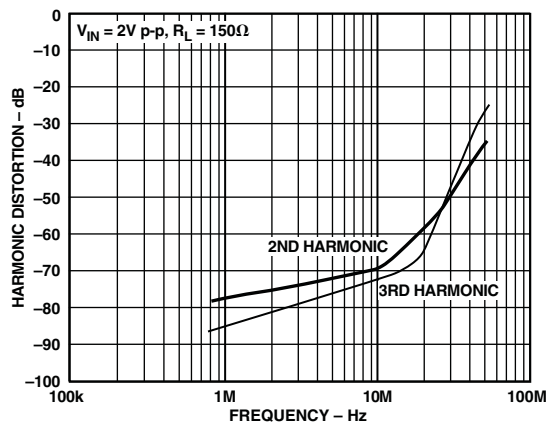
TPC 3. Total Harmonic Distortion
