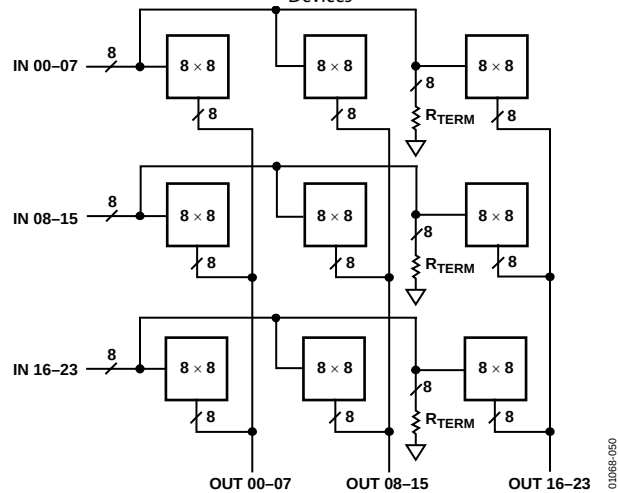
Figure 50. 24 \times 24 Crosspoint Array Using Nine AD8108 Devices or AD8109 Devices
