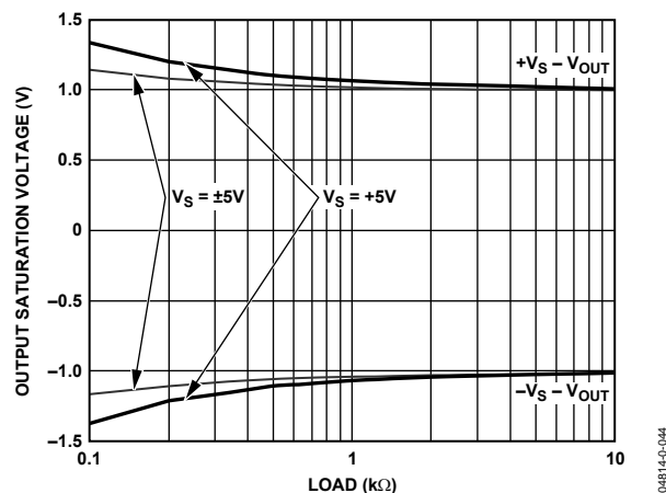
Figure 58. Output Saturation Voltage vs. Load for Various Supplies
