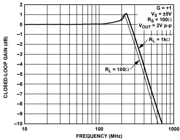
Figure 14. Large Signal Frequency Response for Various Loads
