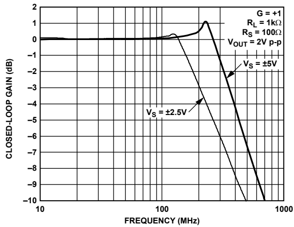
Figure 13. Large Signal Frequency Response for Various Supplies
