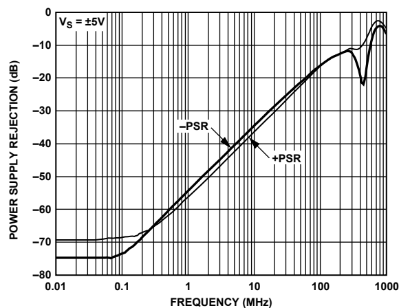
Figure 46. Power Supply Rejection vs. Frequency
