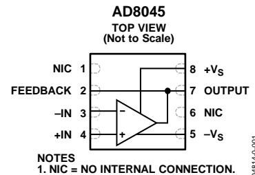
Figure 1. 8-Lead AD8045 LFCSP (CP-8)
