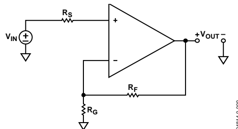
Figure 64. Noninverting Configuration
