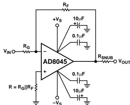
Figure 62. Inverting Configuration
