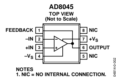
Figure 2. 8-Lead AD8045 SOIC/EP (RD-8)
