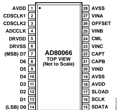
Figure 13. Pin Configuration
