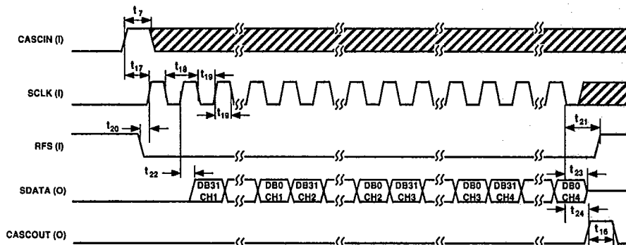
Figure 4. Slave Mode Timing Diagram
