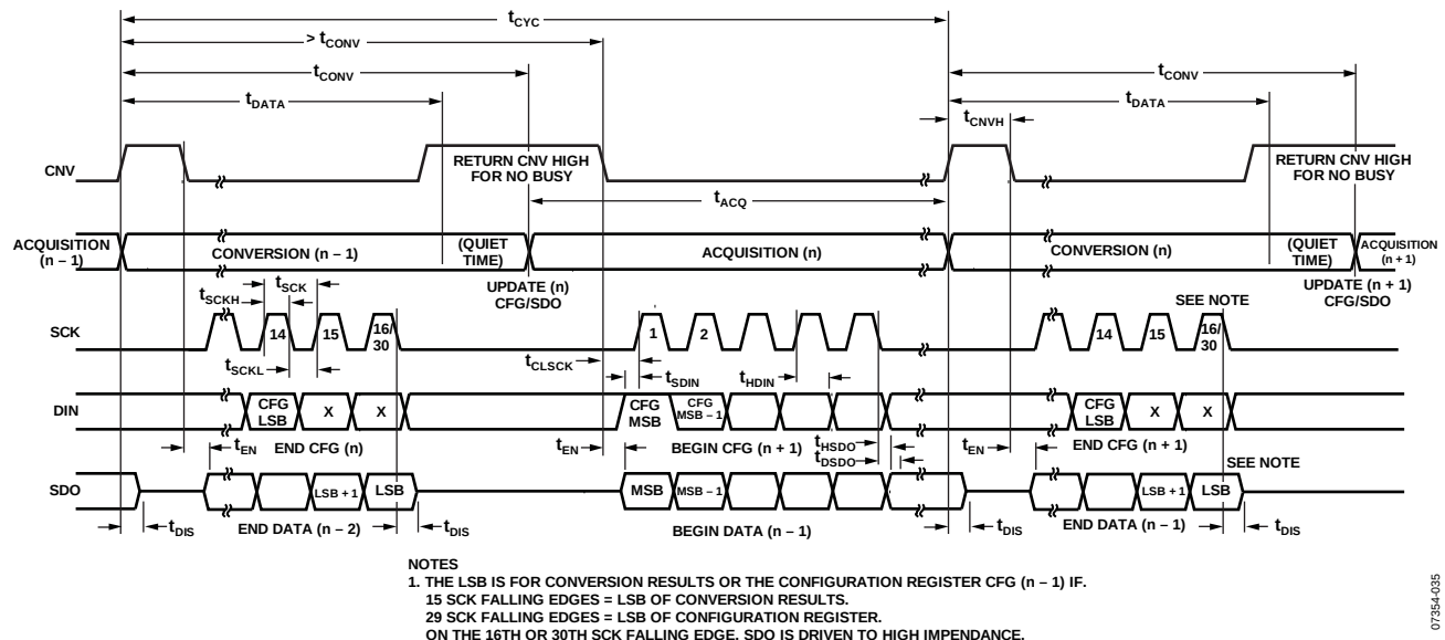
Figure 38. Serial Interface Timing for the AD7699 Without a Busy Indicator
