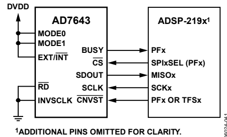
Figure 41. Interfacing the AD7643 to ADSP-219x
