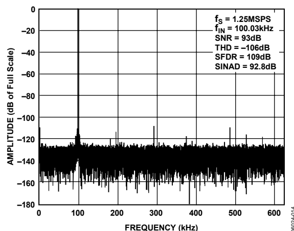
Figure 14. FFT 100 kHz
