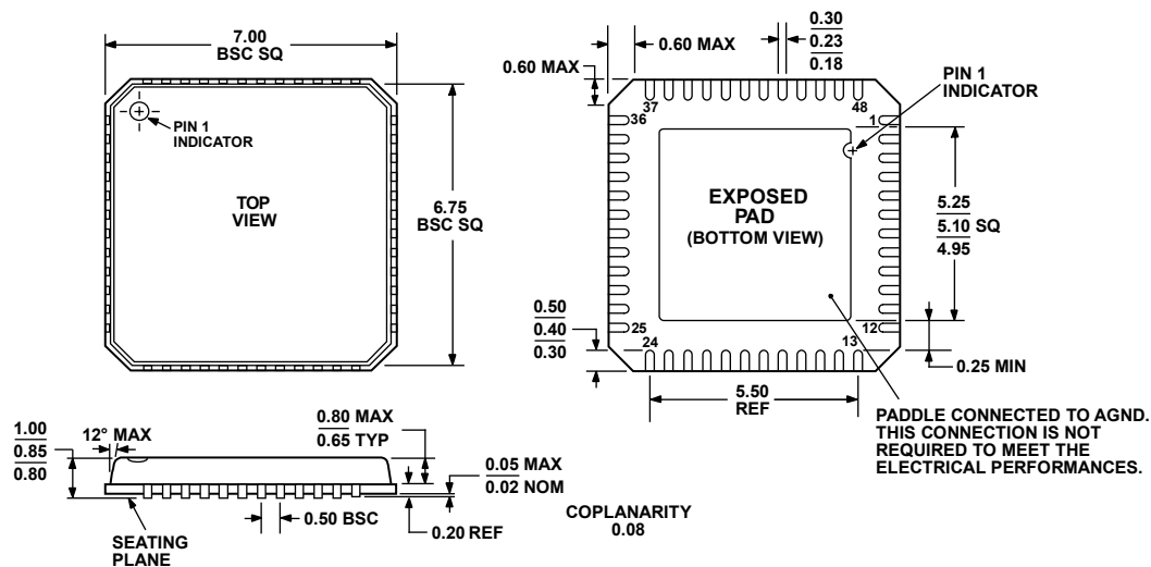
COMPLIANT TO JEDEC STANDARDS MO-220-VKDD-2 Figure 42. 48-Lead Lead Frame Chip Scale Package [LFCSP_VQ] 7 mm × 7 mm Body, Very Thin Quad (CP-48-1) Dimensions shown in millimeters
