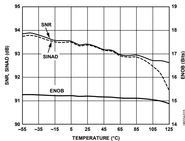
Figure 15. SNR, SINAD, and ENOB vs. Temperature
