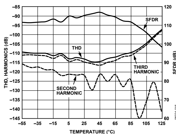
Figure 16. THD, Harmonics, and SFDR vs. Temperature
