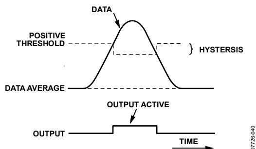
Figure 32. Threshold Hysteresis
