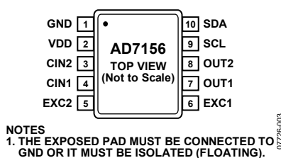
Figure 3. Pin Configuration
